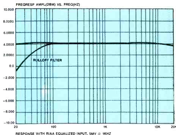
Figure 2. The upper curve shows the frequency response with an RIAA equalized input. The low-frequency rolloff curve also is evident.
