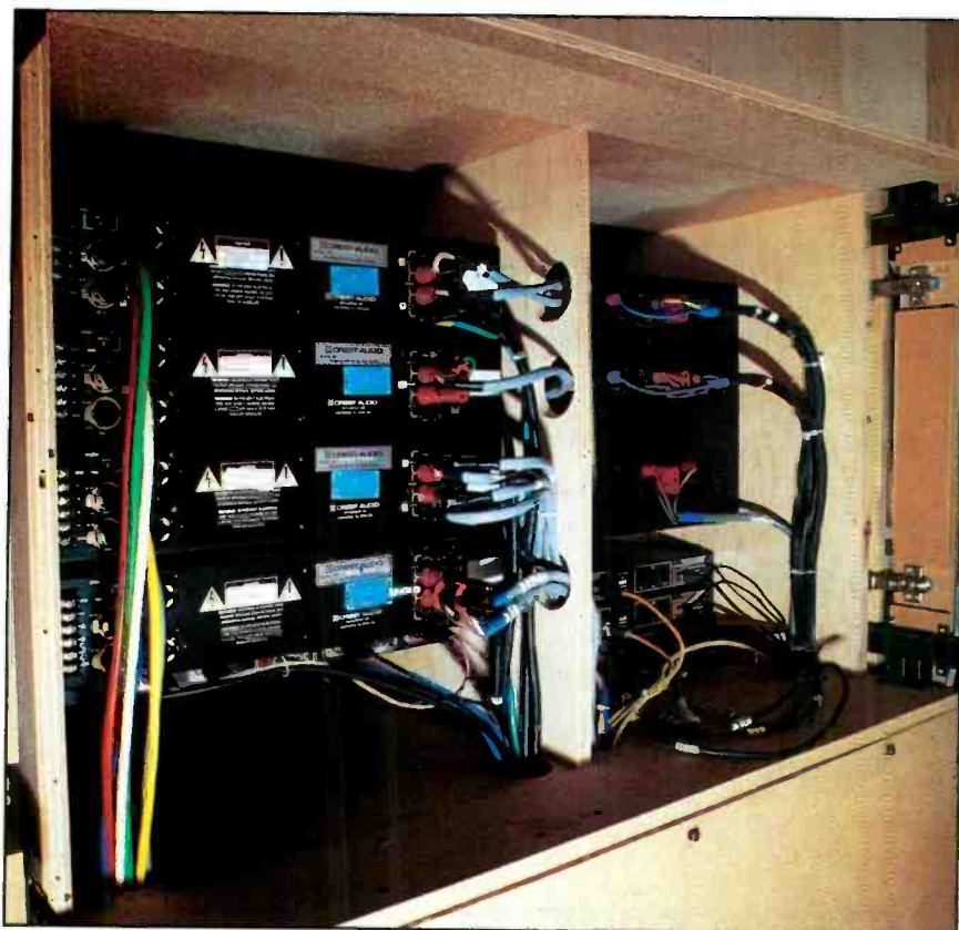
In these high-end systems, the equipment and wiring techniques would make any broadcast engineer proud. (Courtesy of Don Dutkowski.)
