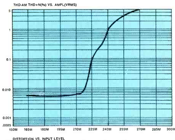
Figure 1. Distortion vs. input level shows an overload point of 240mV.
