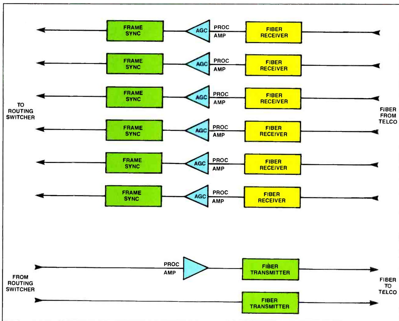
Figure 1. Most signals enter and leave the network on fiber. The six incoming fibers are level set with AGC-equipped proc amps, and then synchronized with frame syncs. The main outgoing line is processed, the backup goes direct. There are four spare fibers.
